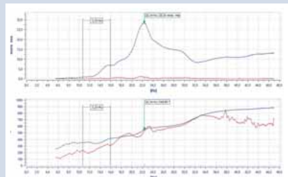
Run-up Bode diagram plot
