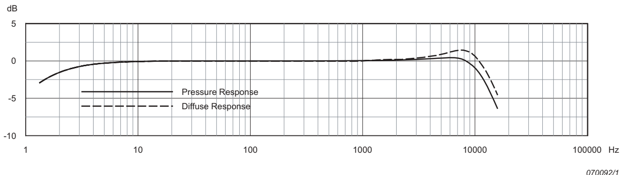
Fig. 1 Typical frequency response of the microphone with protection grid. The low-frequency response is valid when the vent is exposed to the sound field
