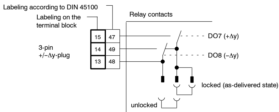
Figure 4-3 Circuit
