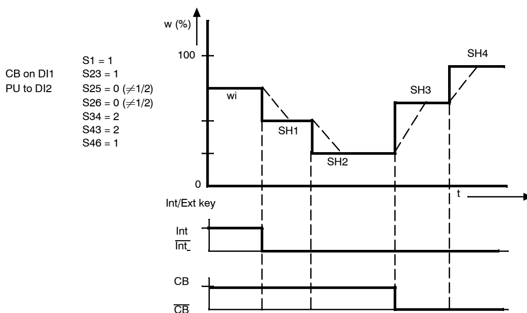
Figure 7-3 Setpoint curve with and without setpoint ramp (according to example 3)
