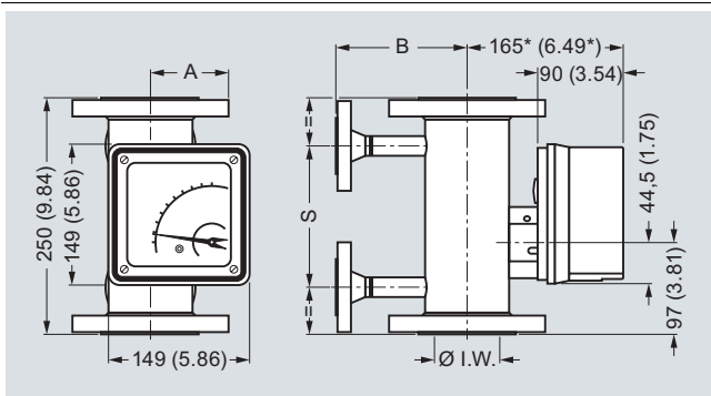
SITRANS FVA250, enclosure of display unit made of aluminum with heating connection, dimensions in mm (inch)
