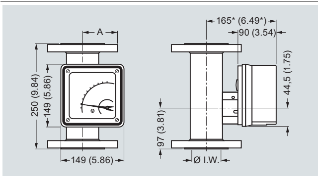
SITRANS FVA250, enclosure of display unit made of aluminum, dimensions in mm (inch)
