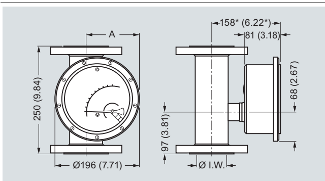
SITRANS FVA250, enclosure of display unit made of stainless steel, dimensions in mm (inch)
